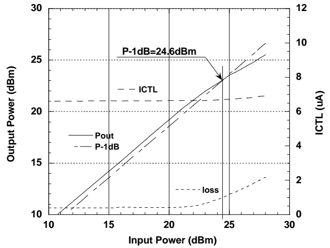
Pin vs. Pout, ICTL and Loss
