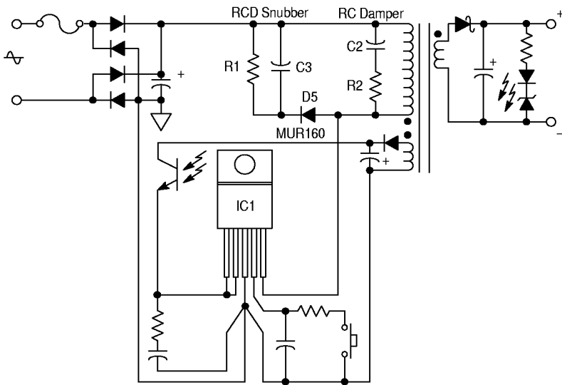
Figure 29. Snubber and Damper Circuits
