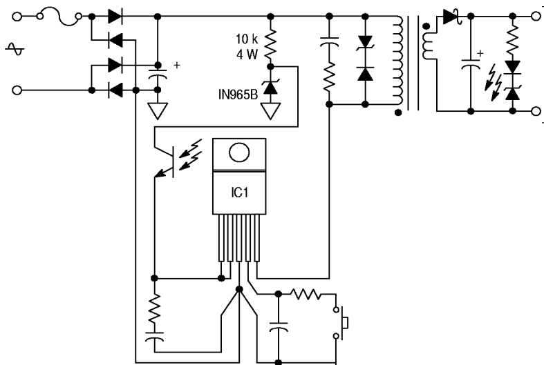
Figure 31. Transformer Auxiliary Winding Elimination Zener Shunt Regulator Method
