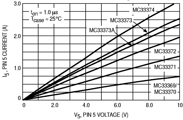
Figure 13. Power Switch Circuit Current versus Pin 5 Voltage
