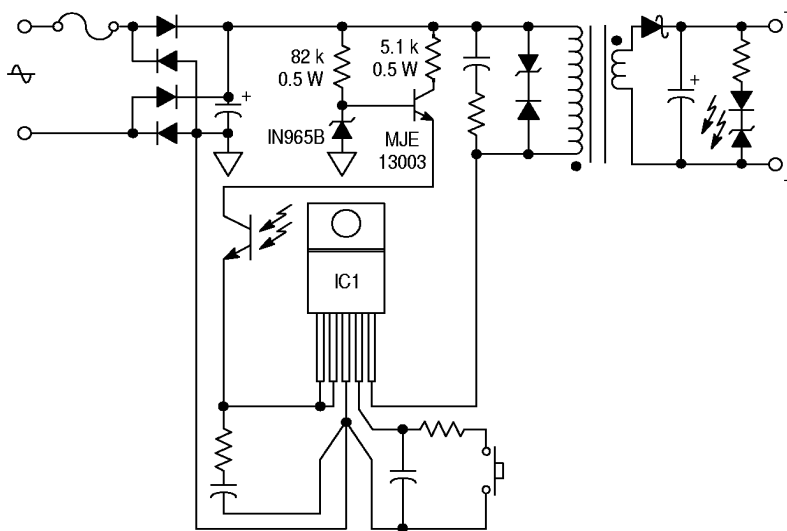
Figure 32. Transformer Auxiliary Winding Elimination Bipolar Transistor Series Regulator Method
