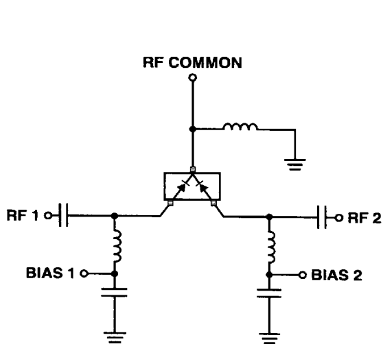
Figure 22. Simple SPDT Switch, Using Only Positive Current.
