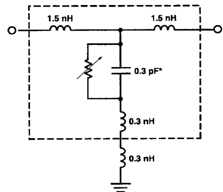
Figure 34. Equivalent Circuit.
