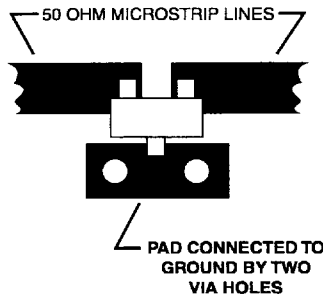
Figure 33. Circuit Layout.
