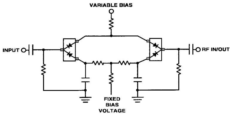
Figure 26. Four Diode \pi Attenuator.
