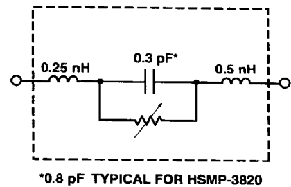
Figure 32. Equivalent Circuit.
