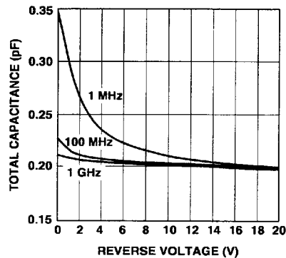
Figure 2. RF Capacitance vs. Reverse Bias, HSMP-3830 Series.
