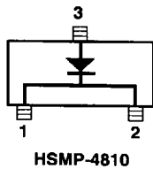
Figure 29. Internal Connections.
