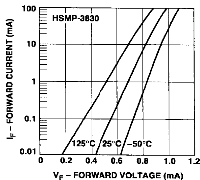
Figure 16. Forward Current vs. Forward Voltage. HSMP-3830 Series.
