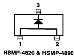
Figure 29. Internal Connections.
