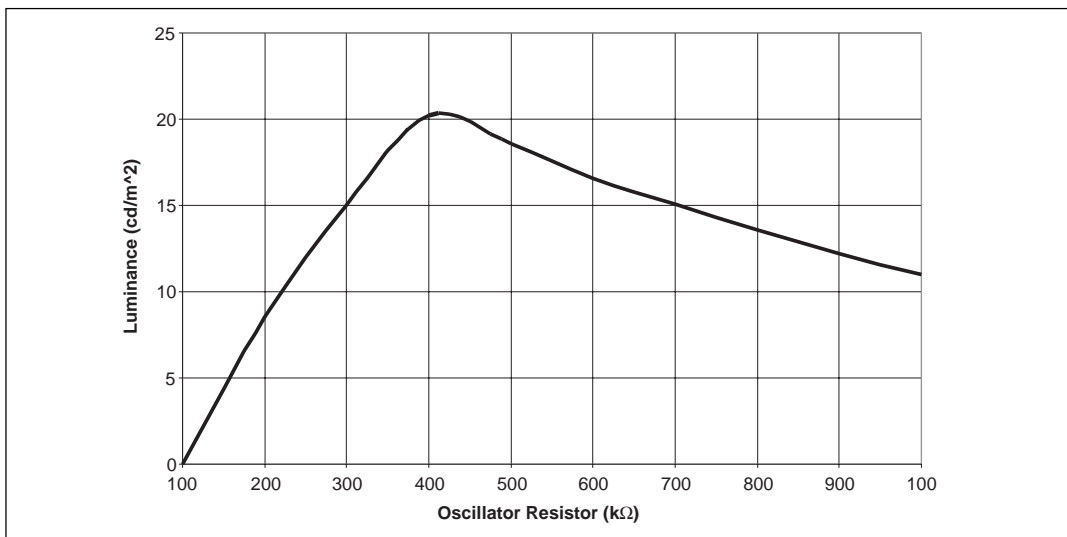
Figure 13. Luminance ( \text{cd/m}^2 ) vs R_{osc}
