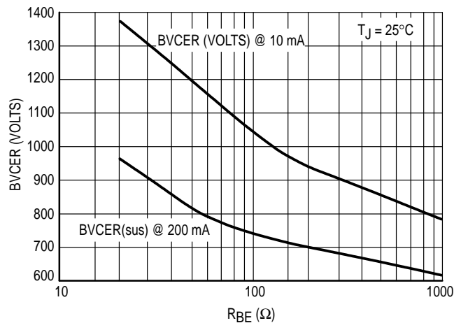
Figure 16. BV_{CEr} = f(R_{BE})
