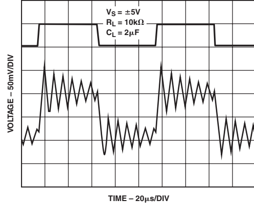
Figure 7. OPA627 Capacitive Load Drive, A_V = +2
