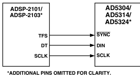
Figure 33. AD5304/AD5314/AD5324 to ADSP-2101/ADSP-2103 Interface
