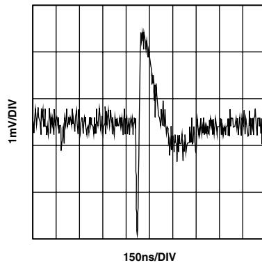
Figure 26. DAC-to-DAC Crosstalk
