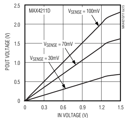
MULTIPLIER TRANSFER CHARACTERISTICS
