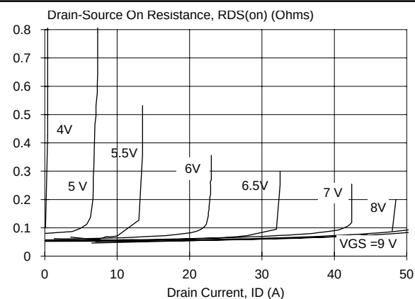
Fig.6. Typical on-state resistance, T_j = 25^\circ\text{C} . R_{DS(ON)} = f(I_D)
