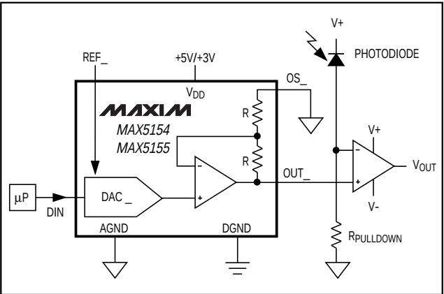
Figure 13. Digital Calibration
