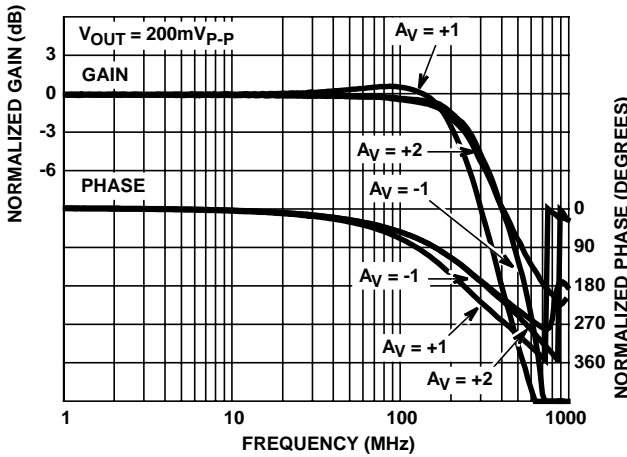
FIGURE 18. FREQUENCY RESPONSE
