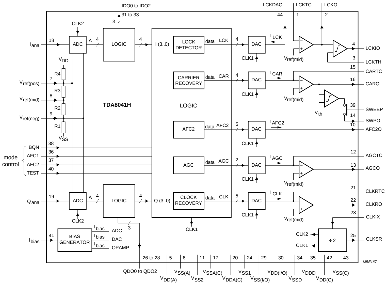
Fig.1 Block diagram.
