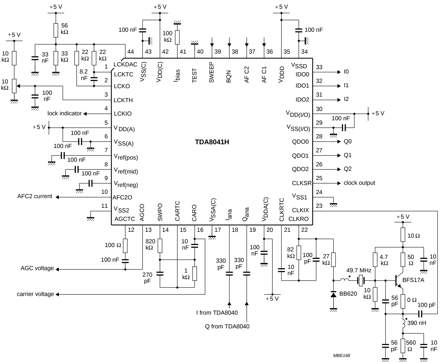
Fig.7 Application diagram.
