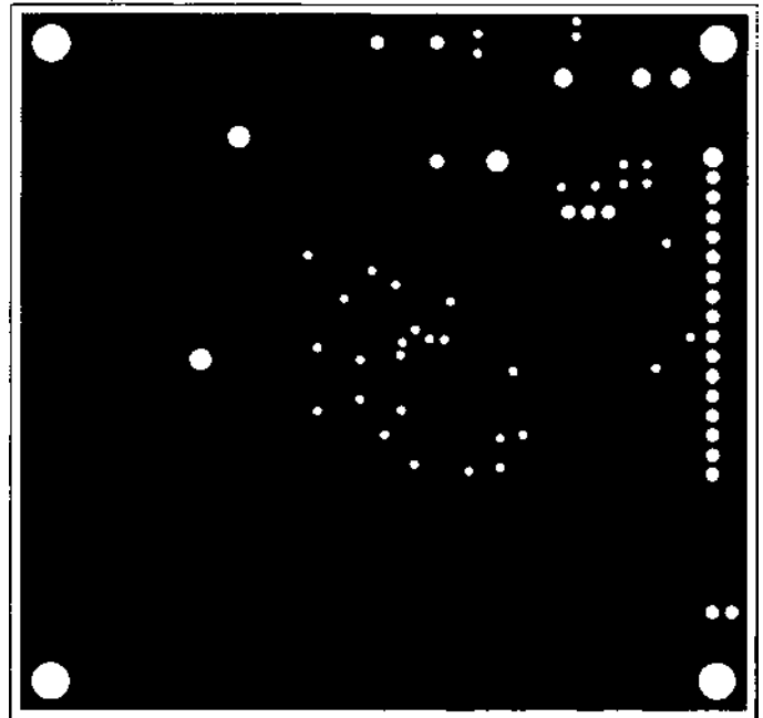
Figure 16. Ground Plane Layer 2 and 5
