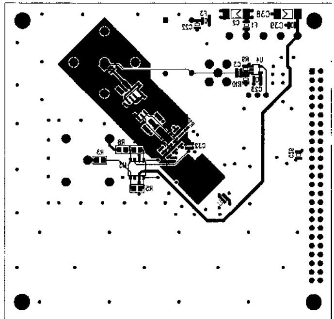
Figure 17. Bottom Signal Layer
