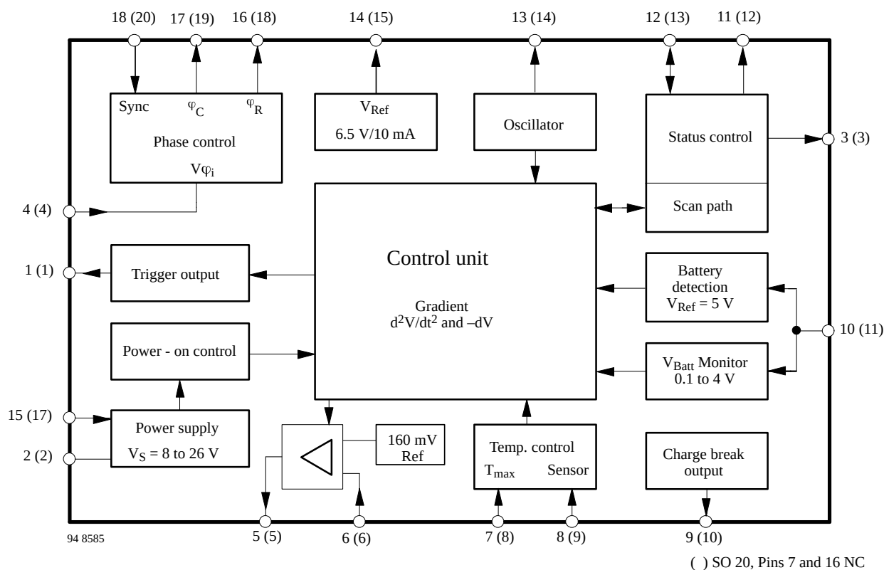
Figure 1. Block diagram
