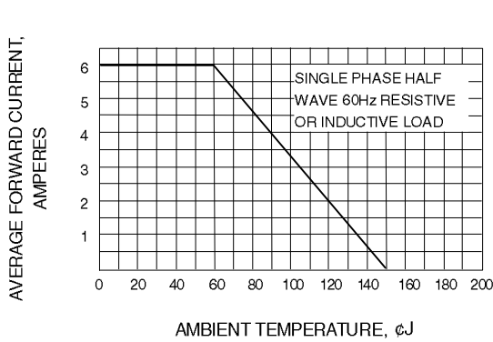
Fig. 2-FORWARD DERATING CURVE
