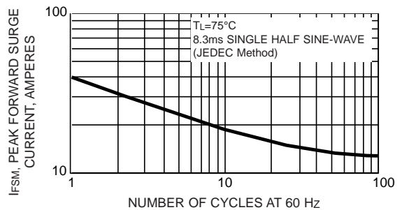
FIG. 6 - MAXIMUM NON-REPETITIVE FORWARD SURGE CURRENT
