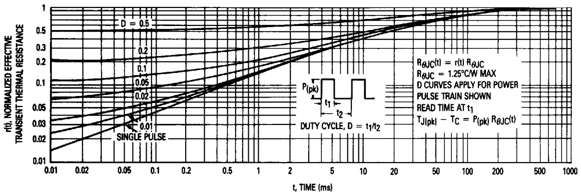
Figure 10. Thermal Response
