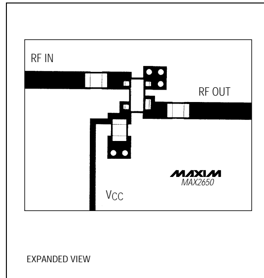
Figure 1. Example PC Board Layout
