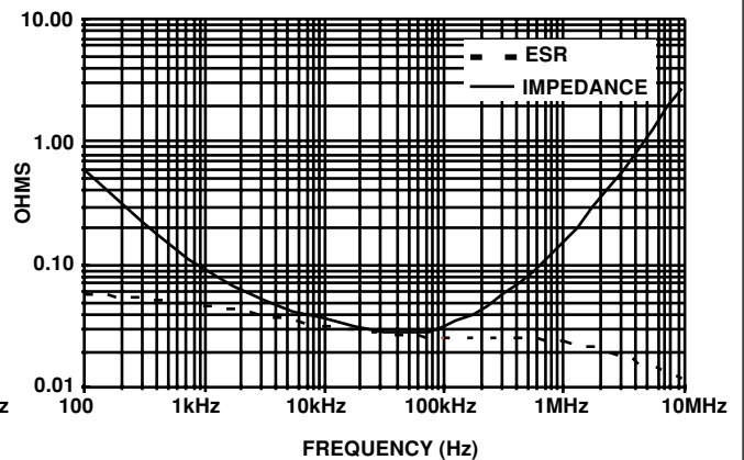
592D 2200-4V Y CASE ESR/IMPEDANCE VS FREQUENCY
