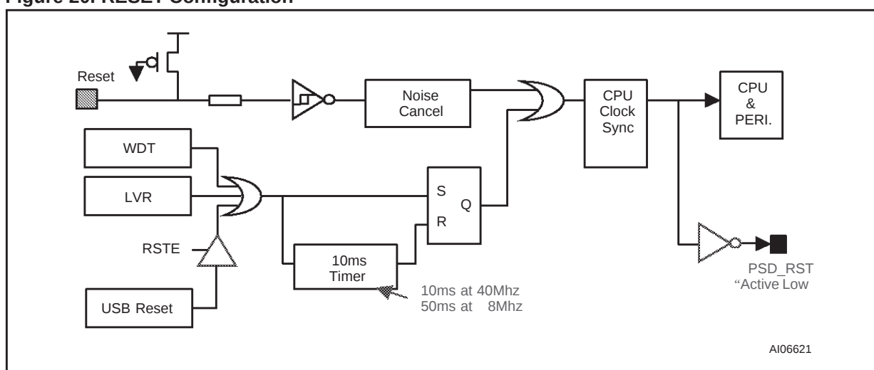
Figure 20. \overline{\text{RESET}} Configuration
