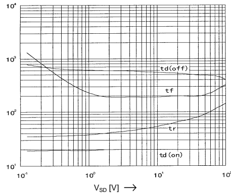
Typical Switching Characteristics
