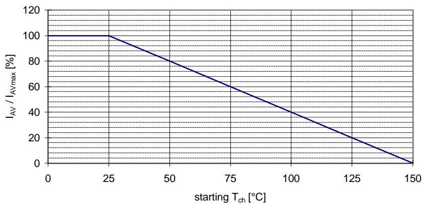
Maximum Avalanche Current vs. starting T ch
