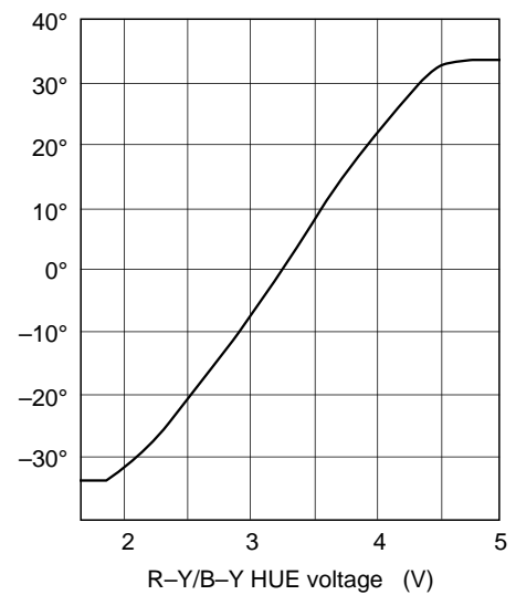
R-Y/B-Y HUE control characteristics
