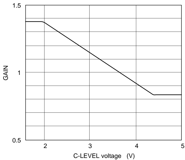
R-Y/B-Y GAIN control characteristics
