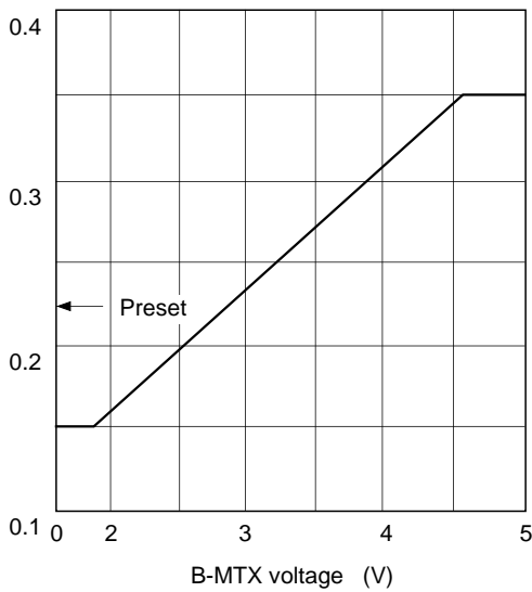
B GAIN control characteristics
