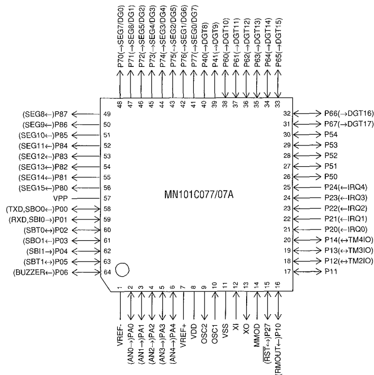
LQFP064-P-1414
