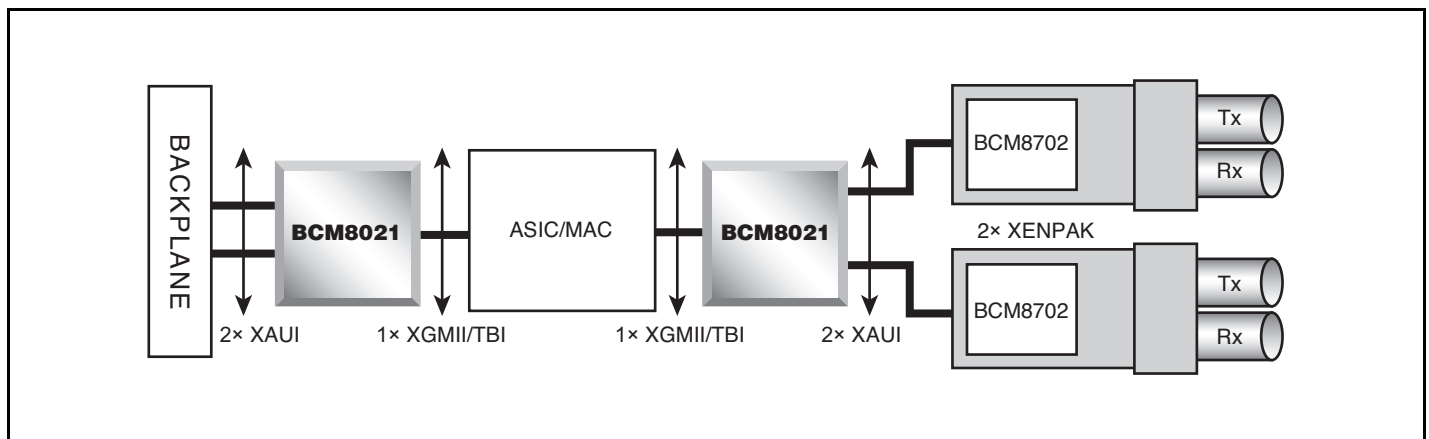
Independent Quad SerDes Application Diagram
