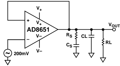
Figure 56. Snubber Network
