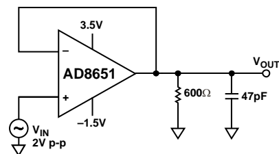
Figure 58. THD + N Test Circuit
